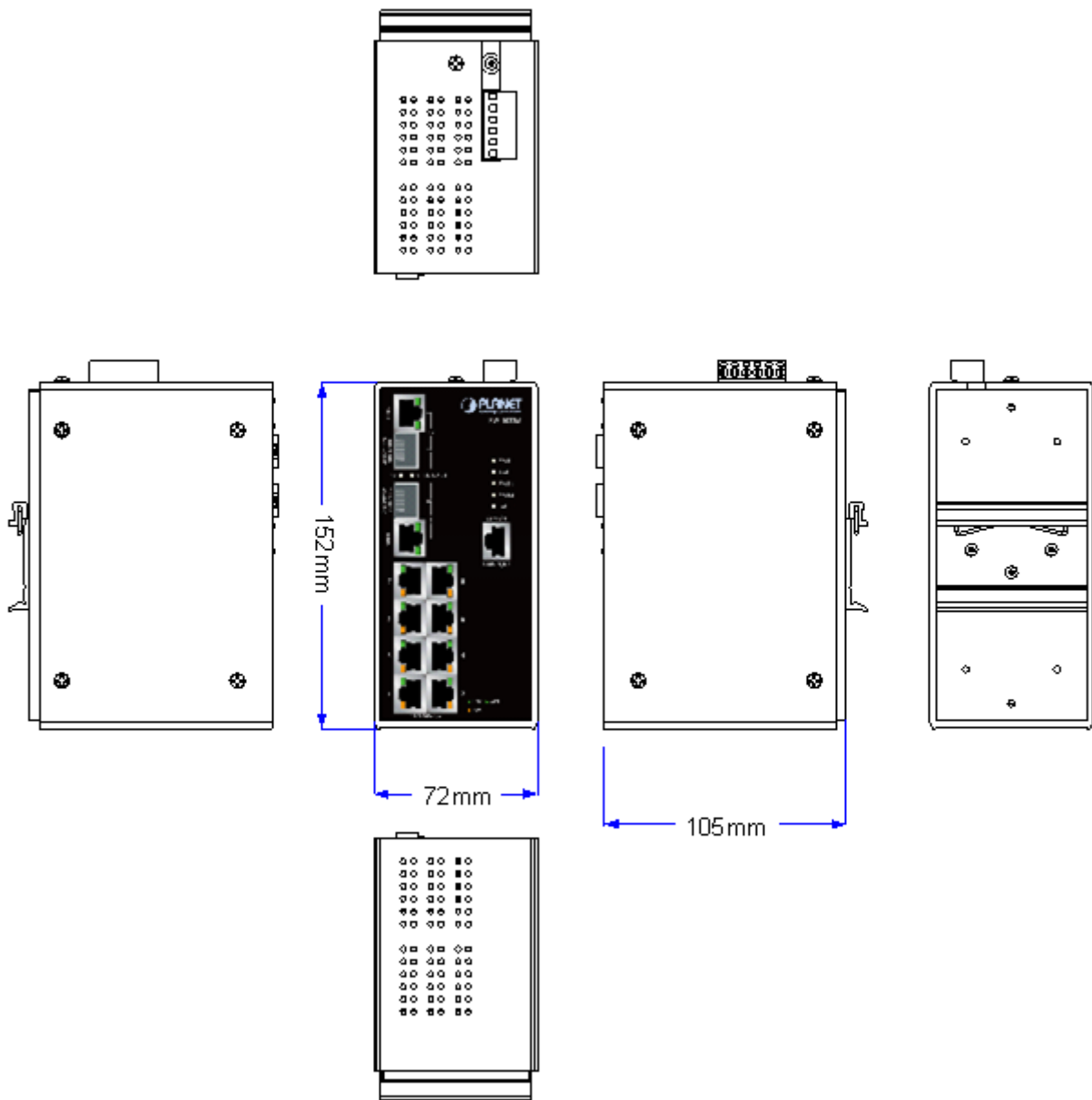
Figure 2-1 ISW-1022M panel layout
