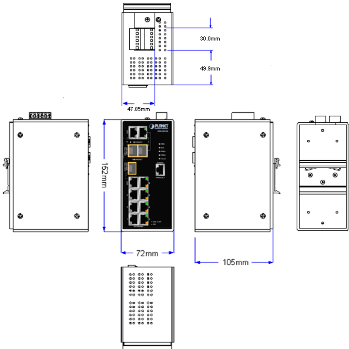
Figure 2-3 ISW-1033MT panel layout
