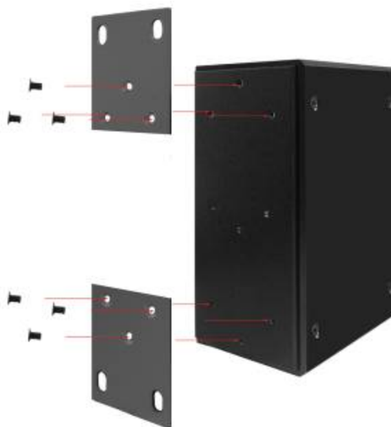
Figure 2-11 Wall mounting
