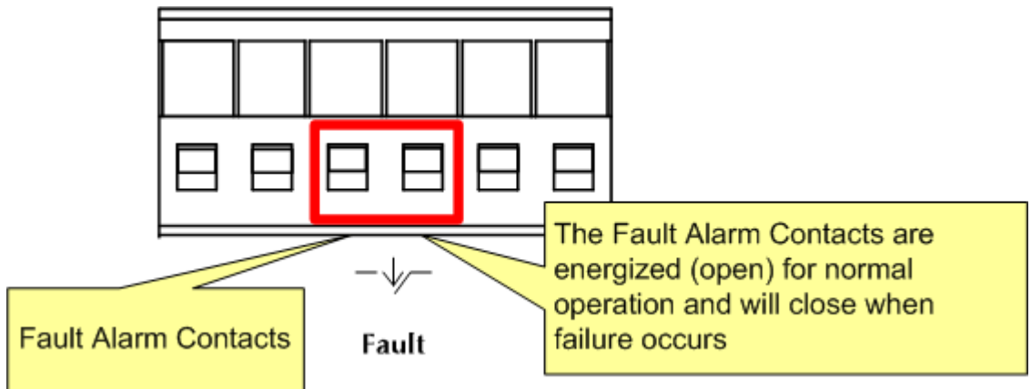
Figure 2-14 Power Fault Alarm trigger description
