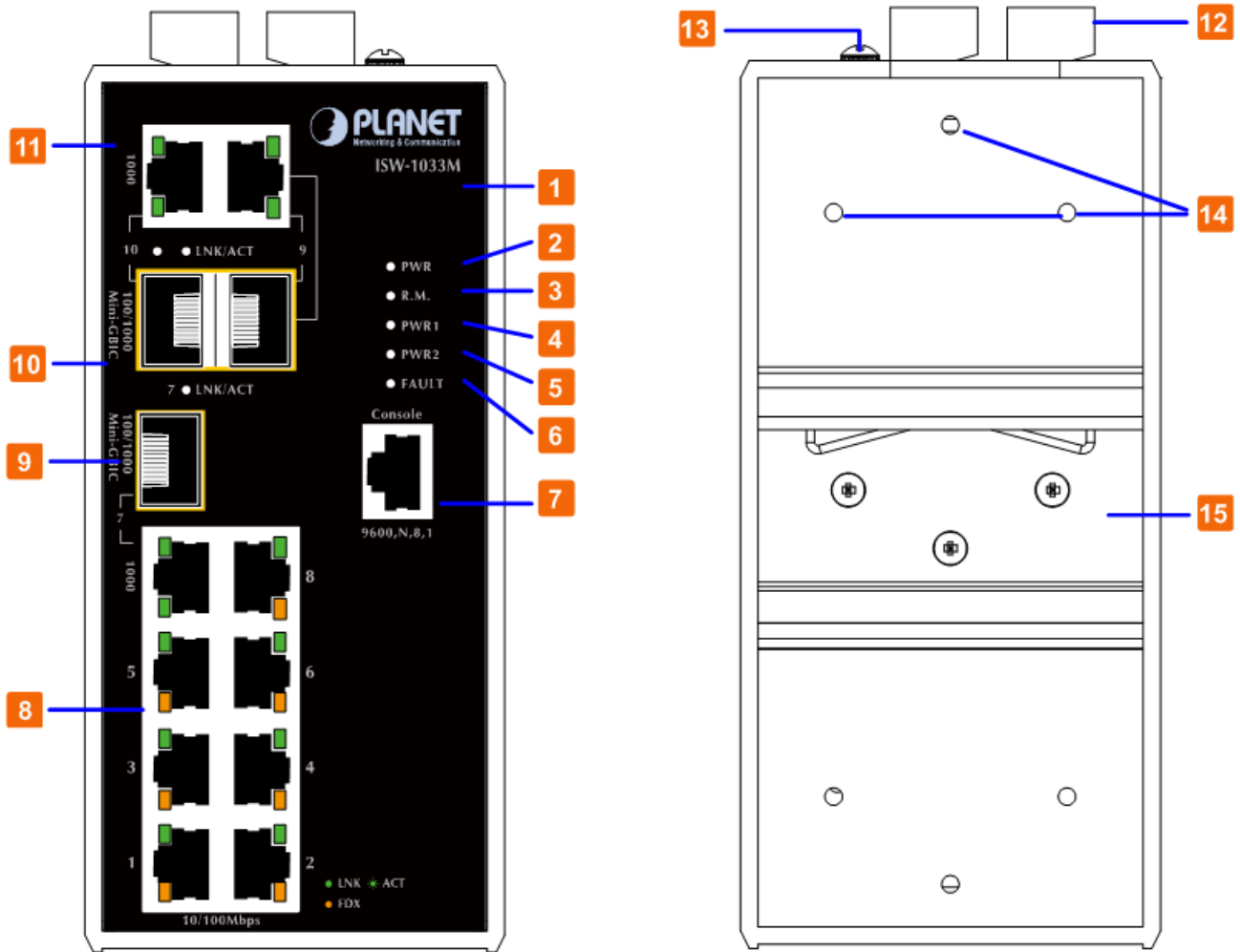
Figure 2-6 Front and Rear Panel of ISW-1033MT
