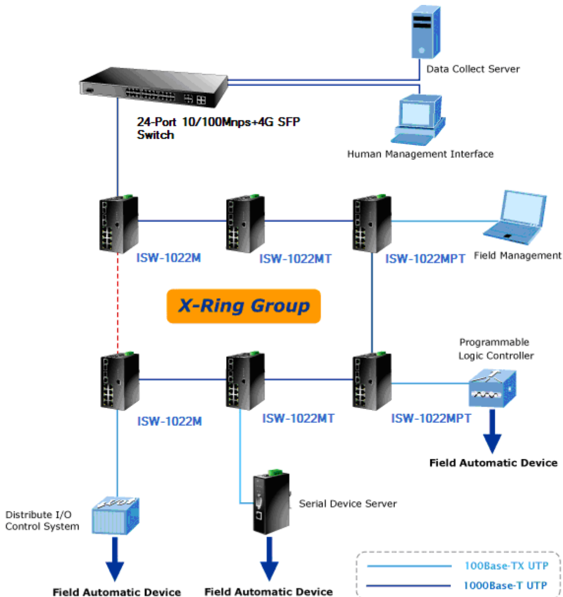
Figure 5-59 X-Ring Application
