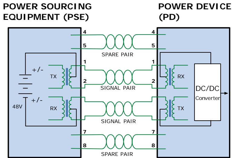
Figure 2 - Power Supplied over the Data Pins
