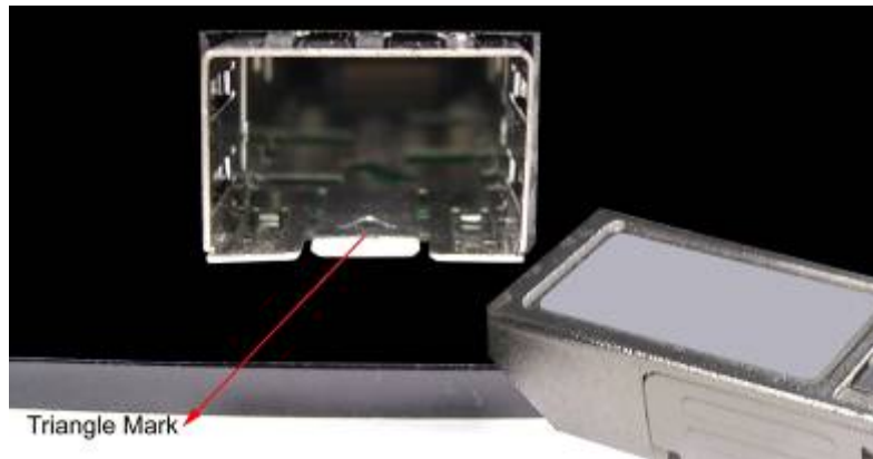
Figure 2-15 Plug-in the SFP transceiver
