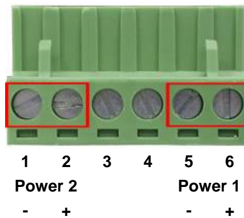
Figure 2-13 6-Pin Terminal Block power wiring input
