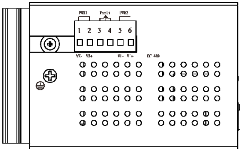
Figure 2-7 Top Panel of ISW-1022MPT
