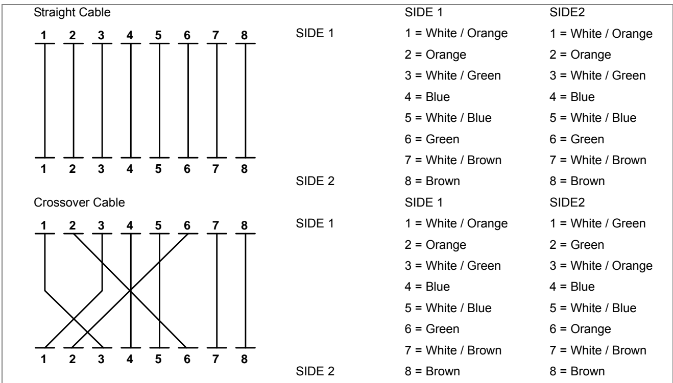
Figure A-1: Straight-Through and Crossover Cable
