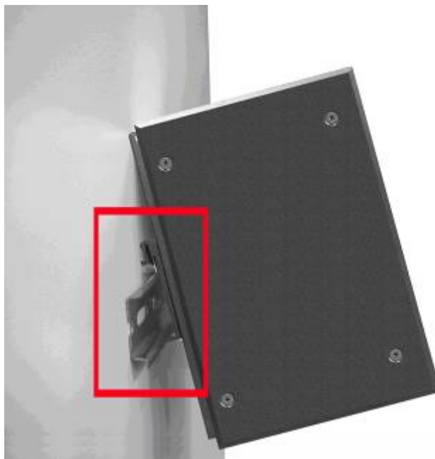
Figure 2-9 DIN-Rail Mounting
