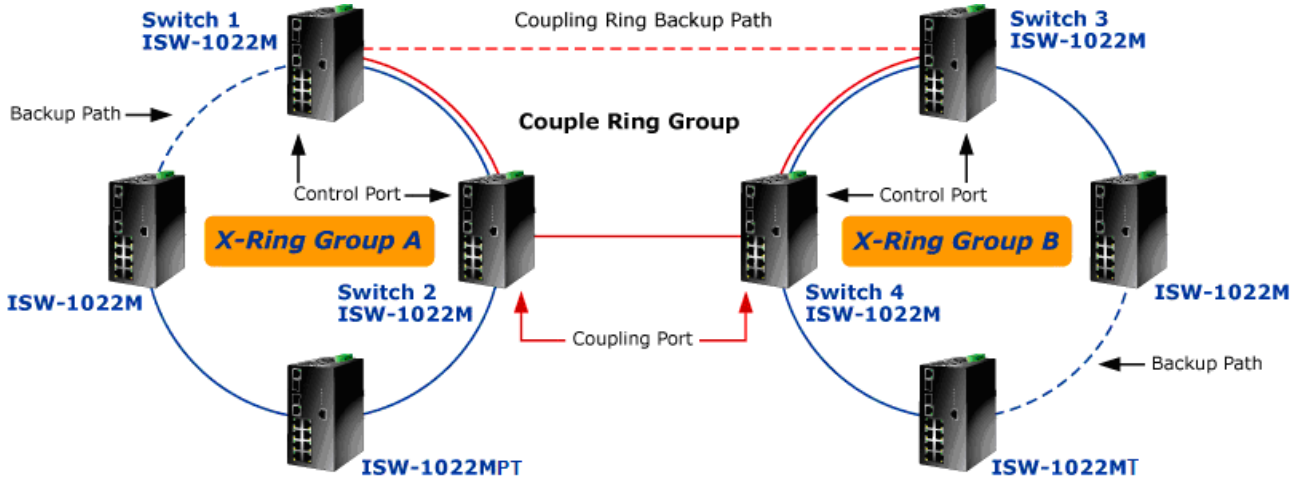
Figure 5-60 Coupling Ring Application
