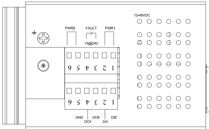
Figure 2-7 Top Panel of ISW-1033MT
