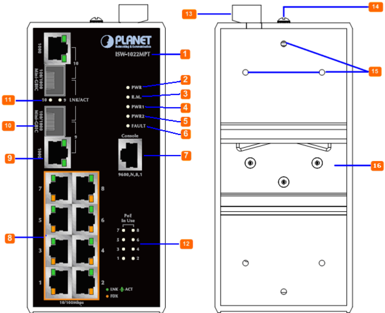
Figure 2-5 Front and Rear Panel of ISW-1022MPT
