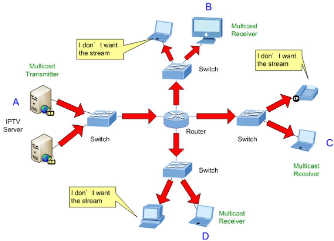
Figure 5-55 Multicast flooding
