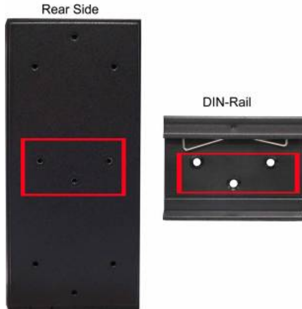
Figure 2-8 Rear Panel – DIN-Rail Kit
