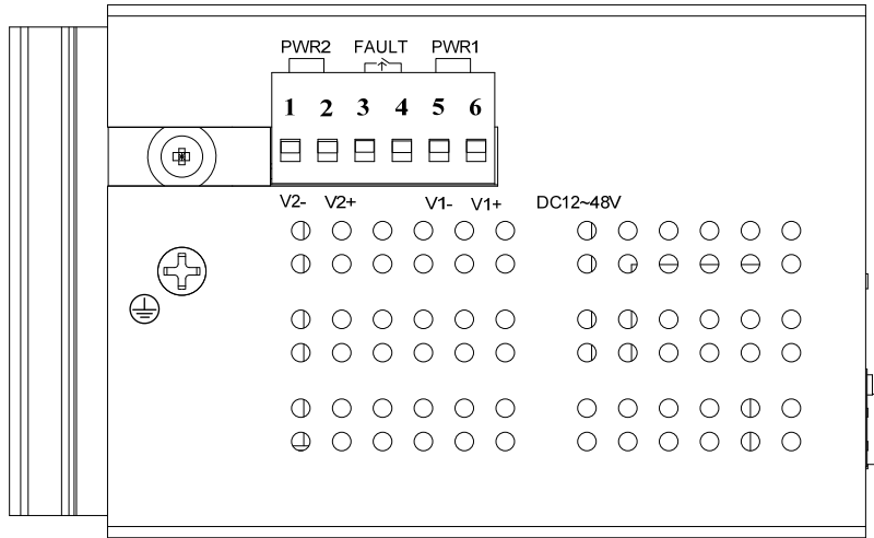
Figure 2-7 Top Panel of ISW-1022M / ISW-1022MT
