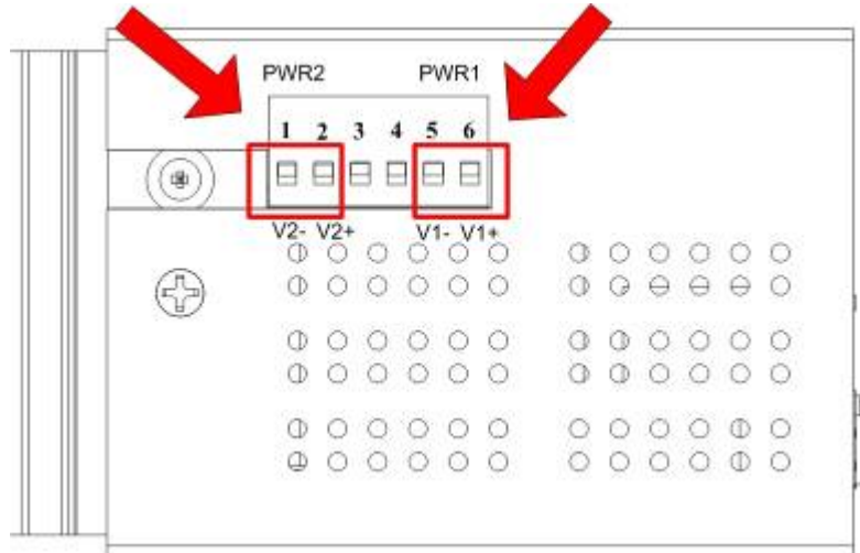
Figure 2-12 Wiring the redundant power inputs
