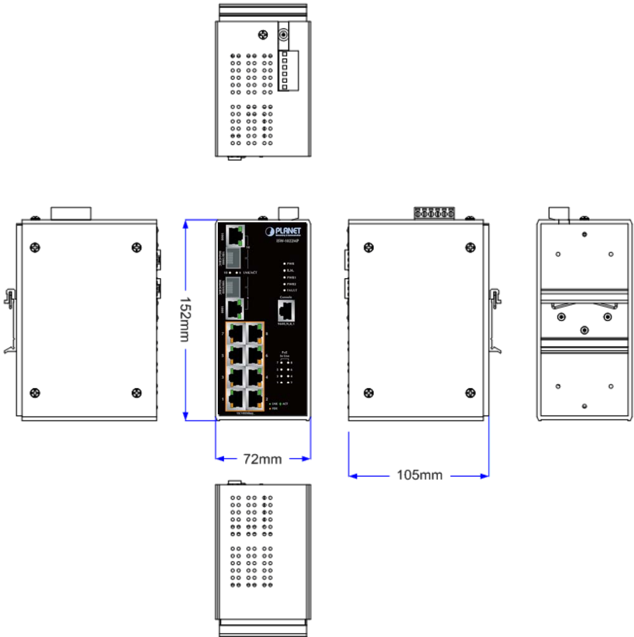
Figure 2-2 ISW-1022MPT panel layout
