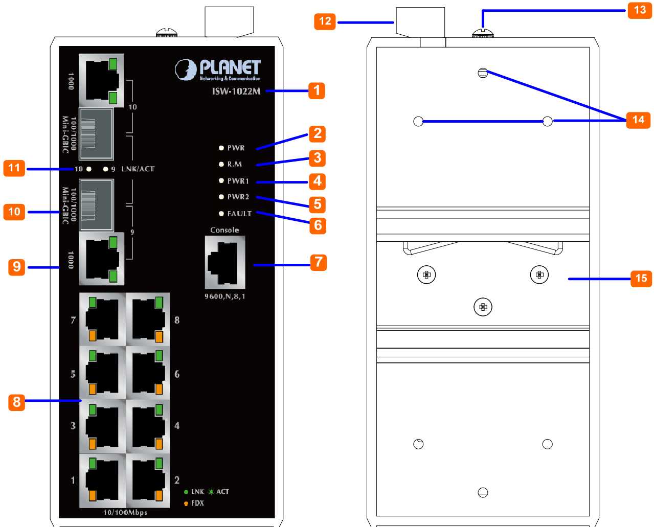
Figure 2-4 Front and Rear Panel of ISW-1022M
