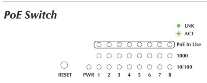
Figure 2-5 PLANET GSD-802PS LED panel
