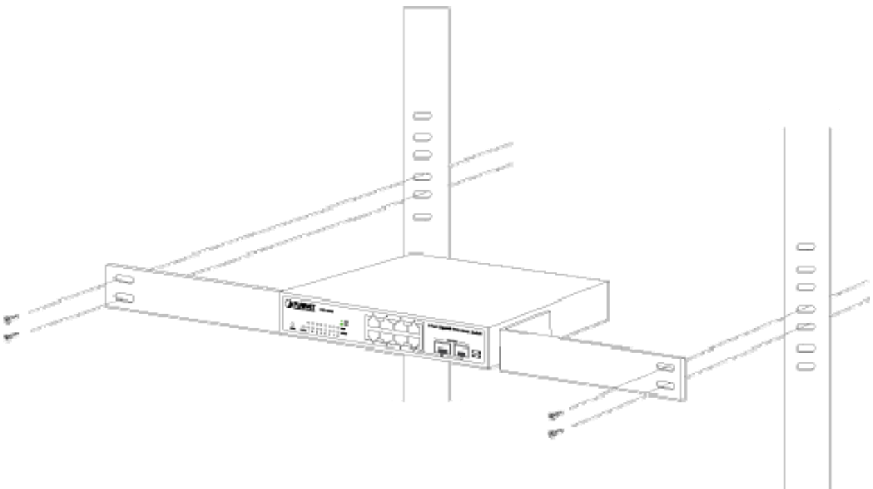
Figure 2-9 Mounting the Gigabit Ethernet Switch in a Rack
