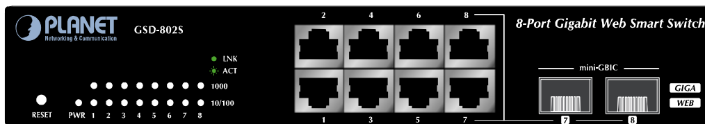
Figure 2-2 PLANET GSD-802S Front Panel
