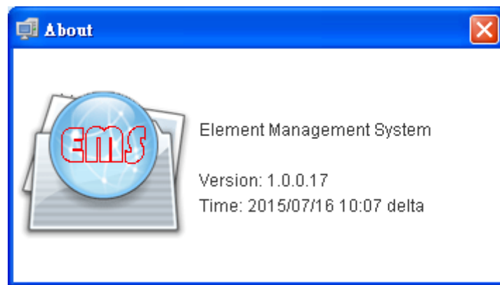
Figure 4-16 About Screen
