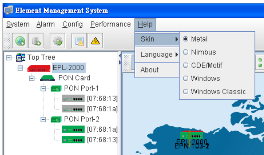
Figure 4-14 Skin Screen
