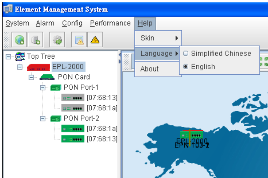
Figure 4-15 Language Screen
