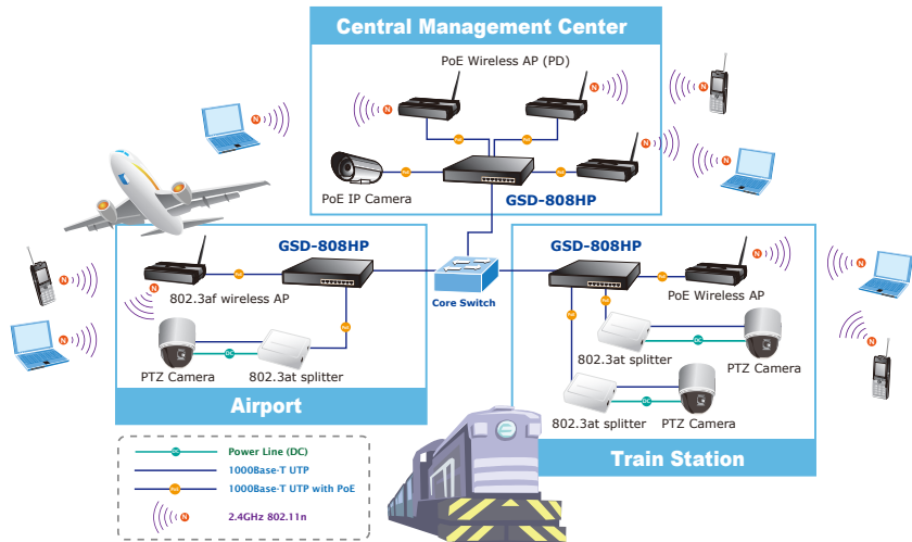
Figure 3-4: Airport / Train Station PoE Switch Connection
