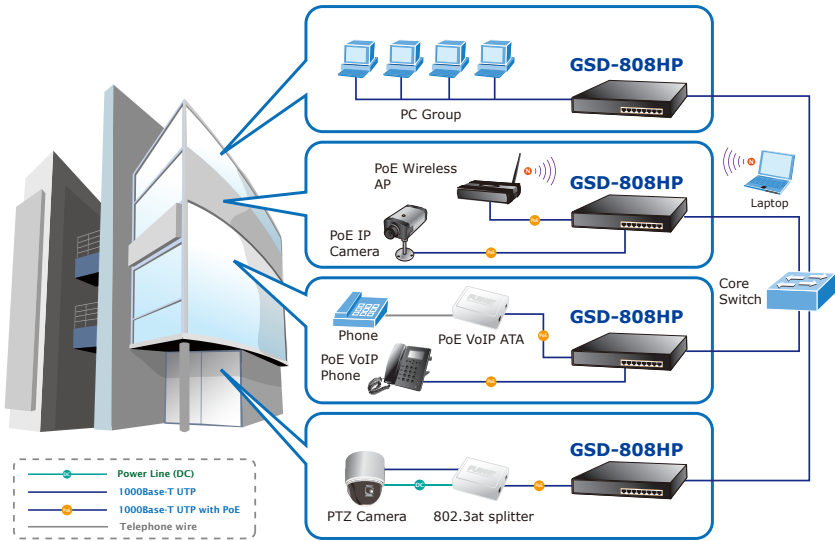
Figure 3-5: IP Office Department / Workgroup PoE Switch Connection
