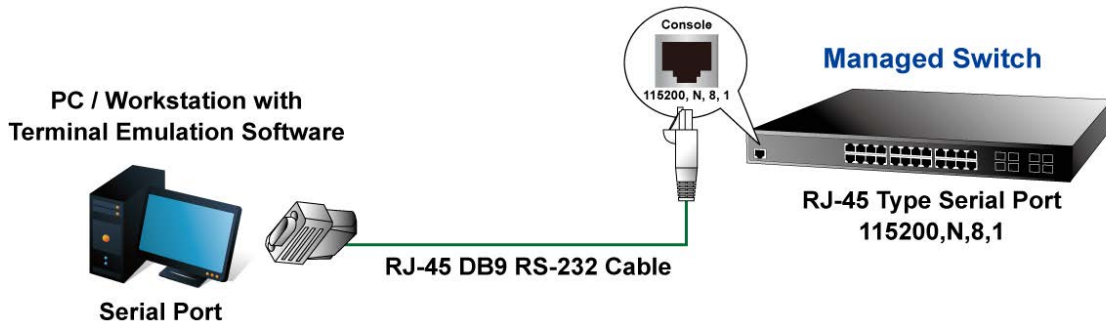
Figure 2-1 Managed Switch Console Connectivity
