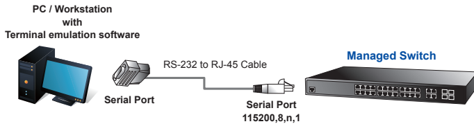
Figure 3-1: Managed Switch Console Connectivity
