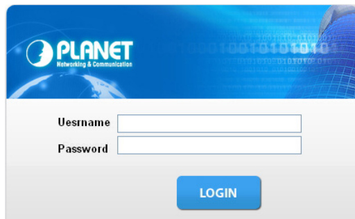
Figure 7-2: Login Screen
