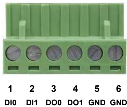
Figure 2-8 6-Pin Terminal Block DI / DO Wiring Input
