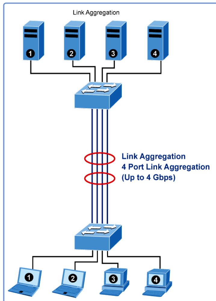
Figure 4-5-1: Link Aggregation
