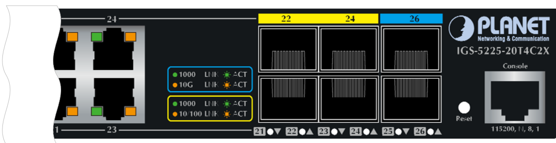
Figure 2-2: Reset Button of Managed Switch
