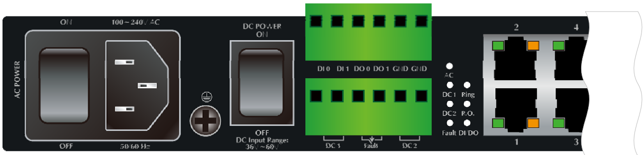
Figure 2-3: IGS-5225-20T4C2X LED on Front Panel
