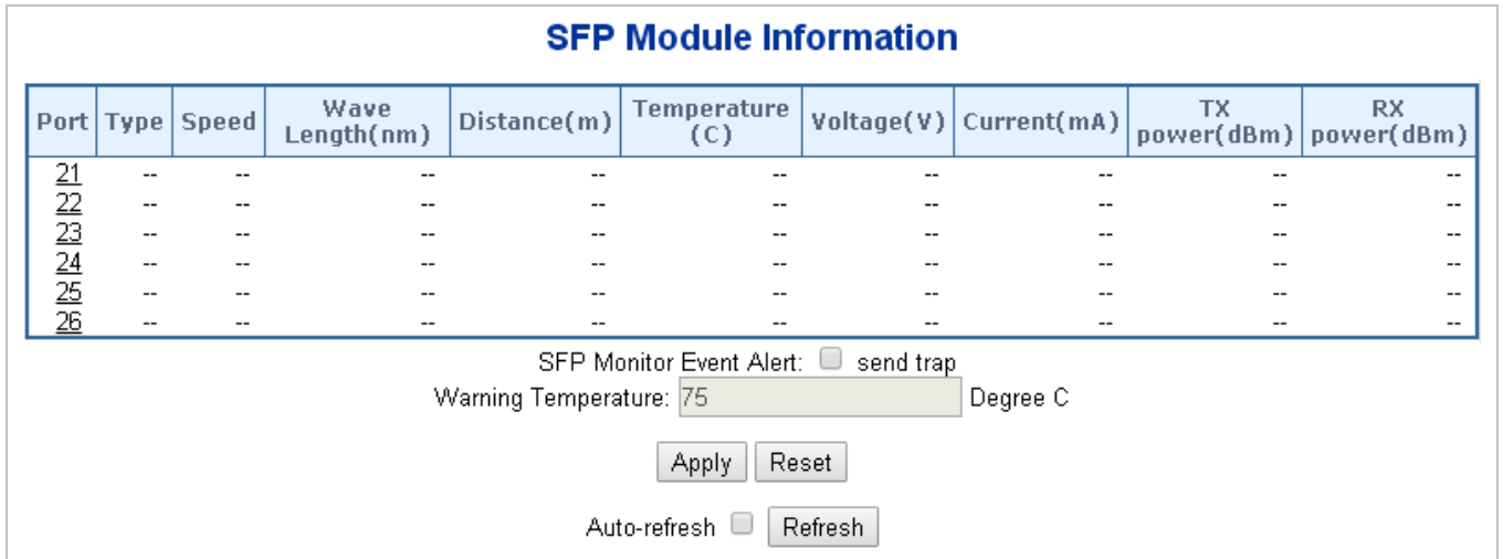
Figure 4-4-4: SFP Module Information for Switch page Screenshot
