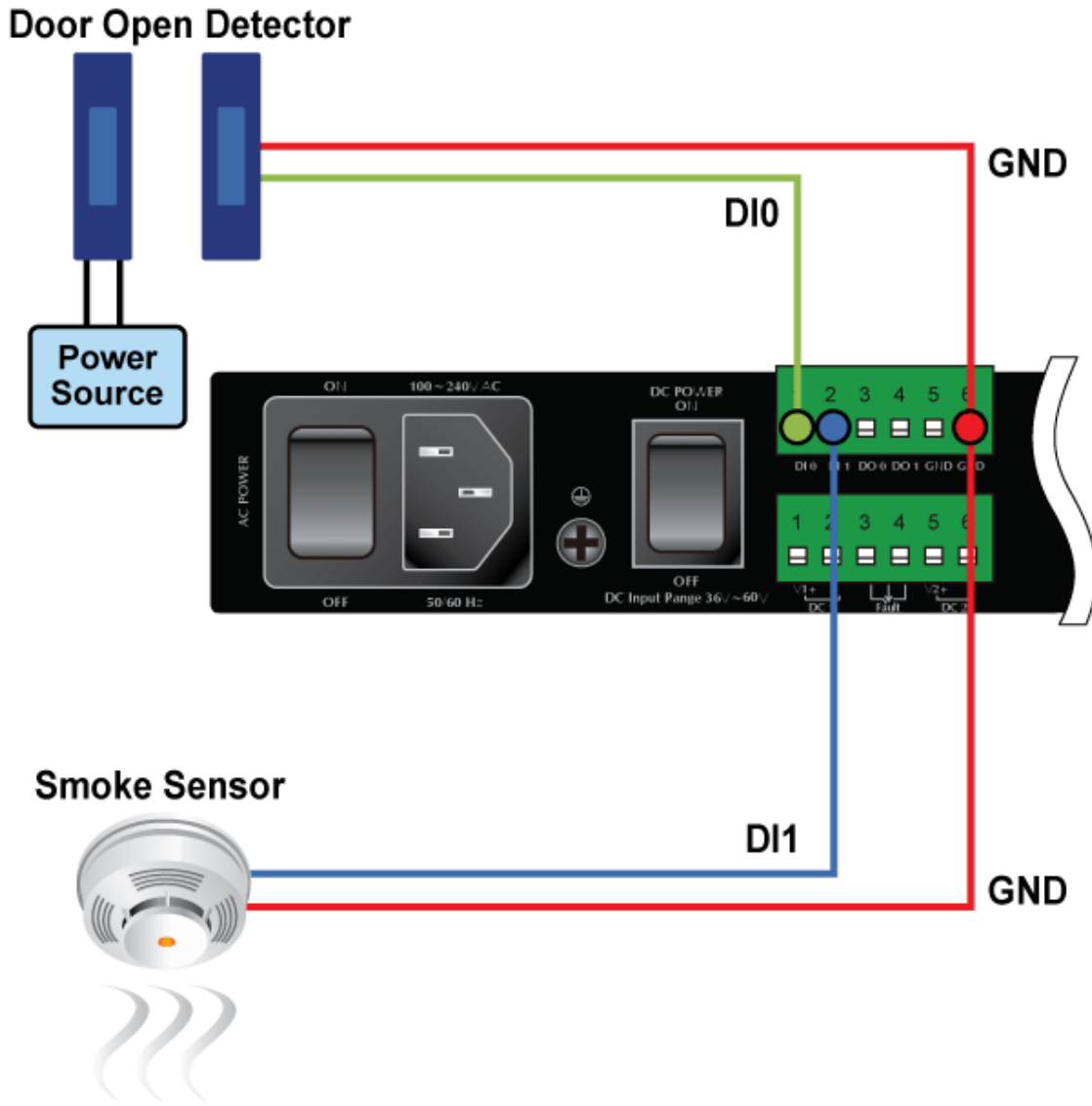
Figure 2-9 Wires DI0 and DI1 to Open Detector
