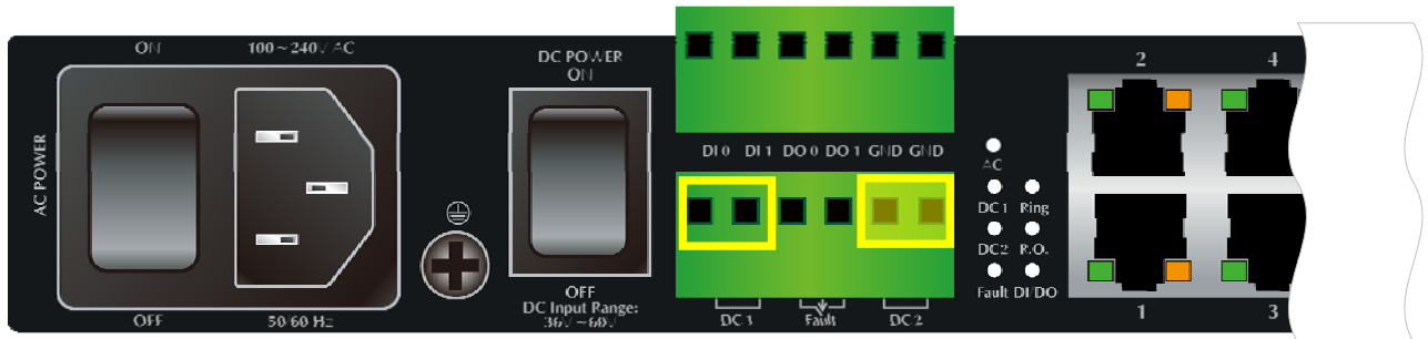
Figure 2-5: IGS-5225-20T4C2X Managed Switch Upper Panel
