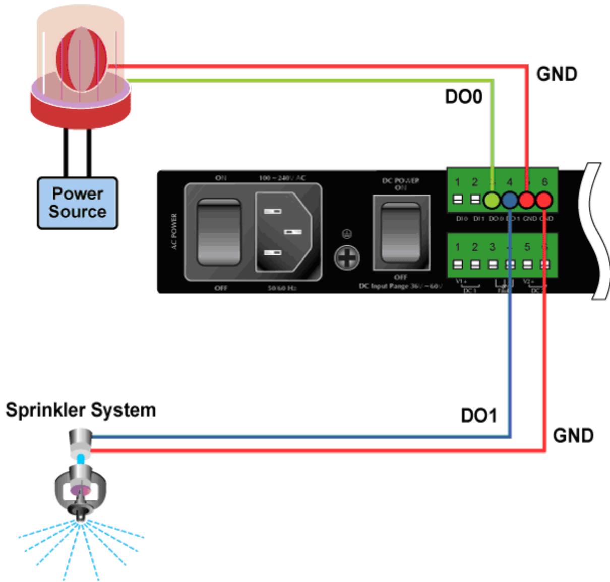
Figure 2-10 Wiring DO0 and DO1 to Open Detector
