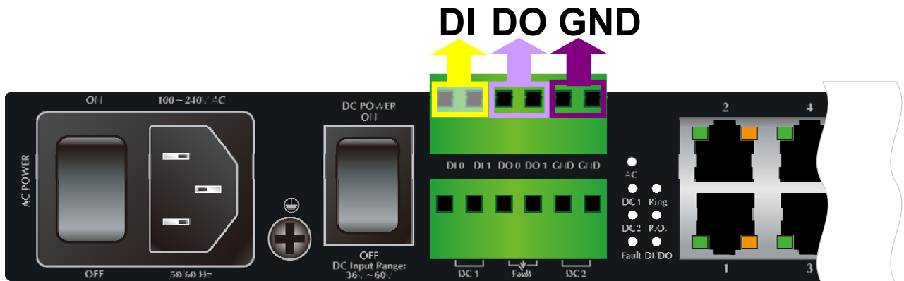
Figure 2-7 Wiring the Redundant Power Inputs
