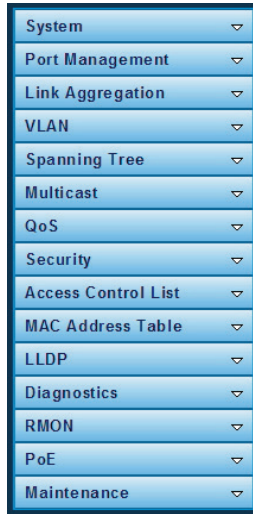
Figure 8-4: Switch Menu
