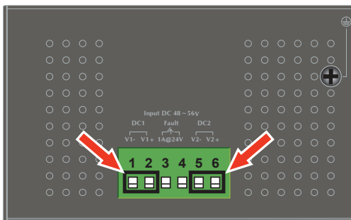
Figure 3-1: IGS-4215-4P4T/IGS-4215-4P4T2S Upper Panel
