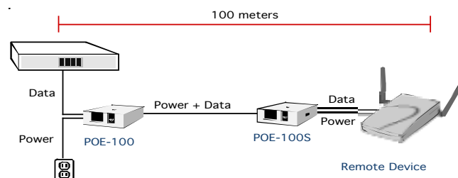
Figure 6: Connection architecture
