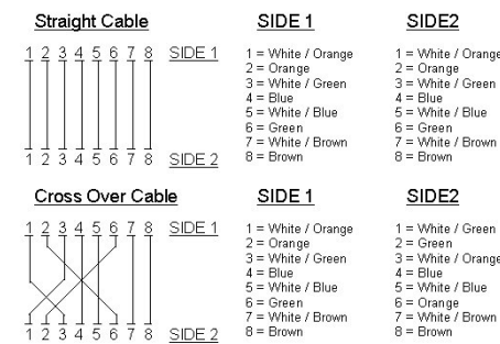
Figure A-2: Straight-Through and Crossover Cable
