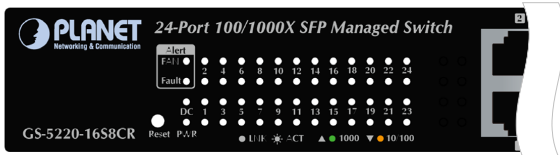
Figure 2-1-13: GS-5220-16S8CR LED on Front Panel
