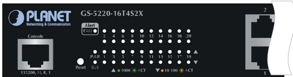
Figure 2-1-14: GS-5220-16T4S2X LED on Front Panel
