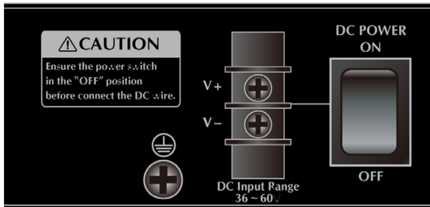
Figure 2-1-16 Rear Panel of GS-5220 redundant power models
