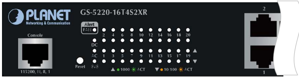
Figure 2-1-15: GS-5220-16T4S2XR LED on Front Panel
