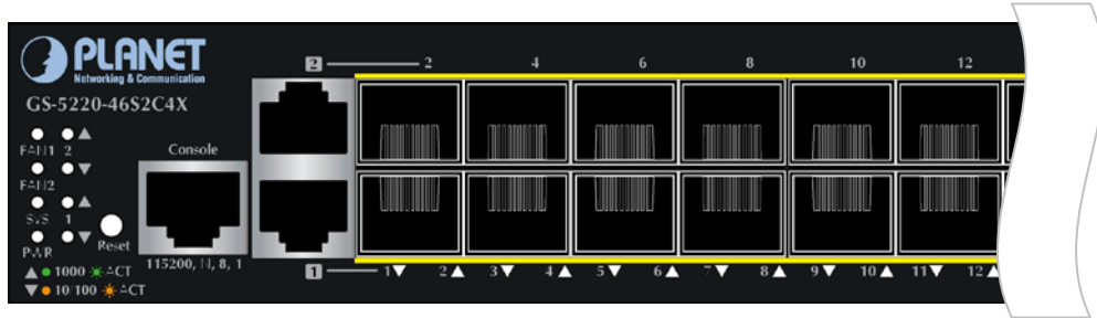
Figure 2-1-19: Front Panel LEDs of GS-5220-46S2C4X
