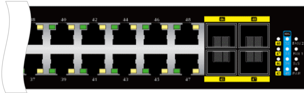
Figure 2-1-20: Front Panel LEDs of GS-5220-48T4X
