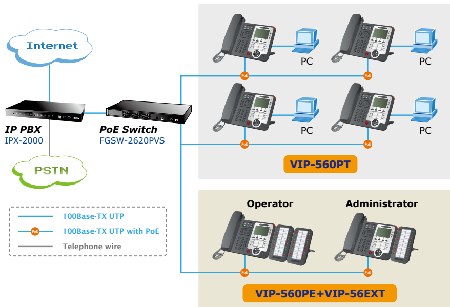
Enterprise IP PBX Deployment : VIP-560PE with VIP-56EXT Expansion Module
