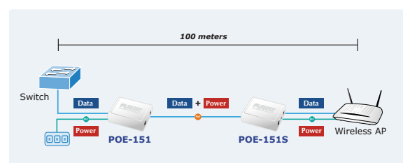
Figure 2: Connection architecture over POE-151/151S
