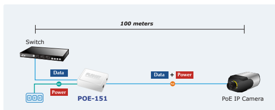
Figure 1: Connection to IEEE 802.3af device
