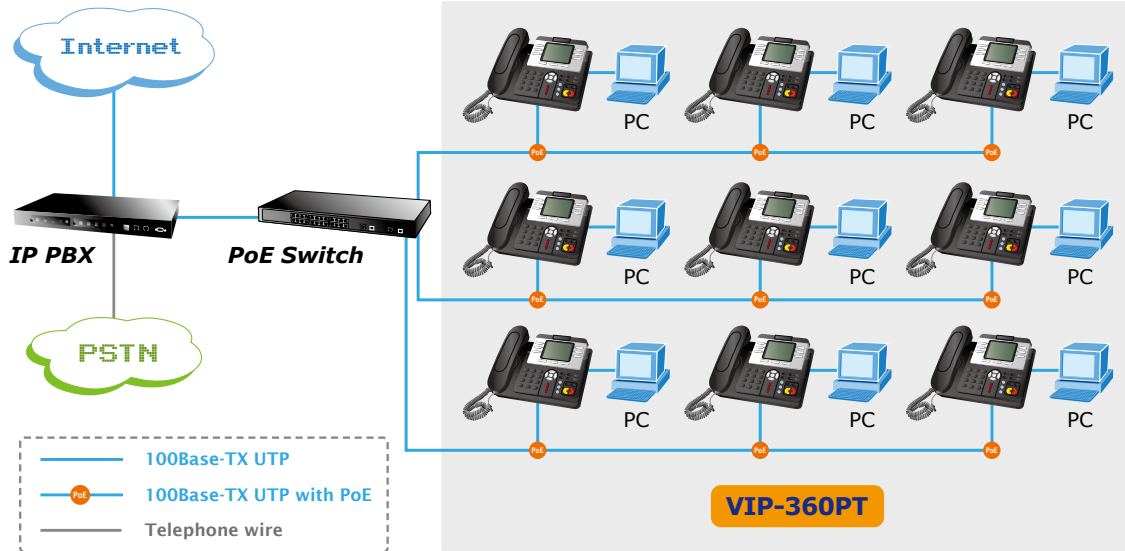
Enterprise IP PBX Deployment with Enterprise PoE IP Phone
