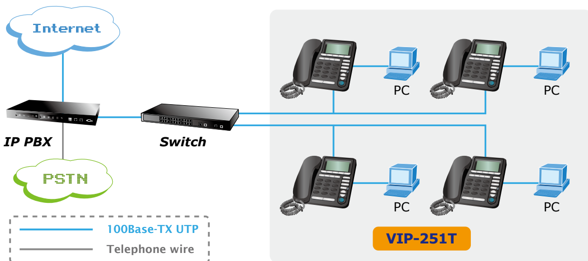
Enterprise IP PBX Deployment with VIP-251T IP Phone
