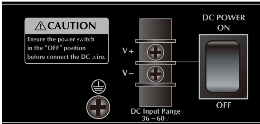
Figure 2-1-34: Rear Panel of GS-5220 PoE series Redundant Power Models
