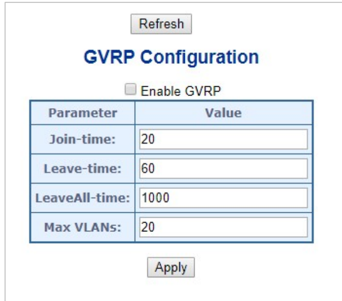
Figure 4-3-12-1: GVRP Configuration Page Screenshot
