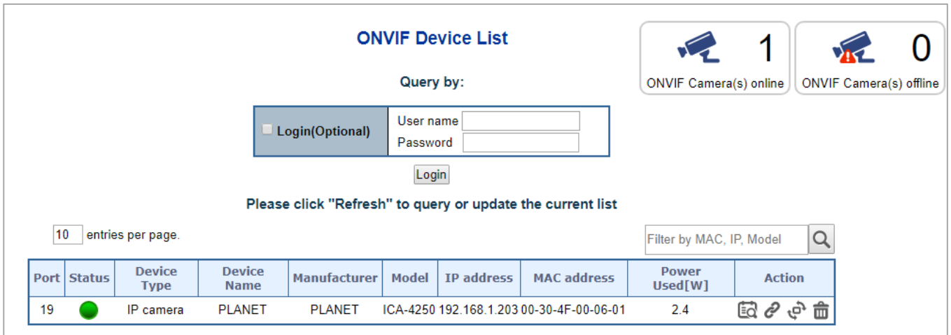
Figure 4-9-1-2: ONVIF Device List Page Screenshot
