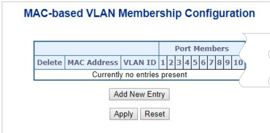
Figure 4-3-3-17: MAC-based VLAN Membership Configuration Page Screenshot
