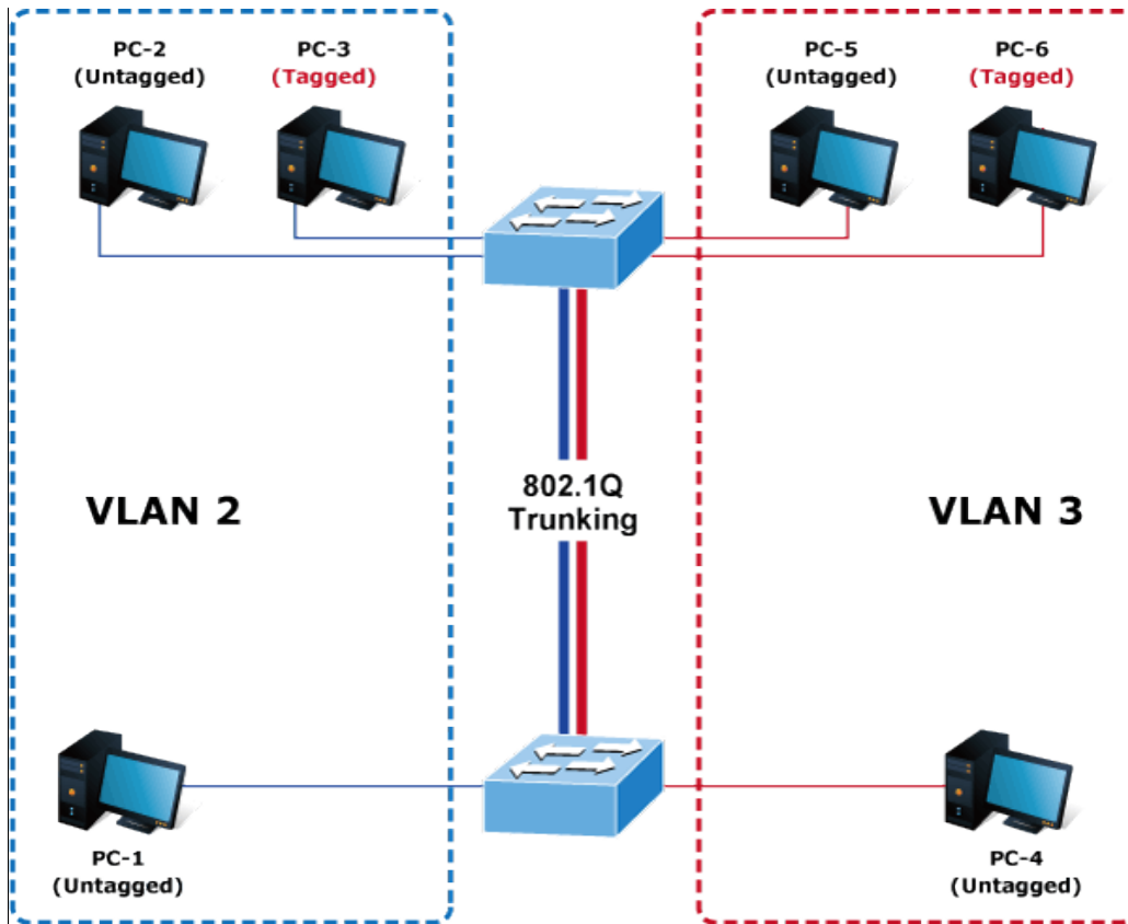
Figure 4-3-3-12: VLAN Trunking Diagram
