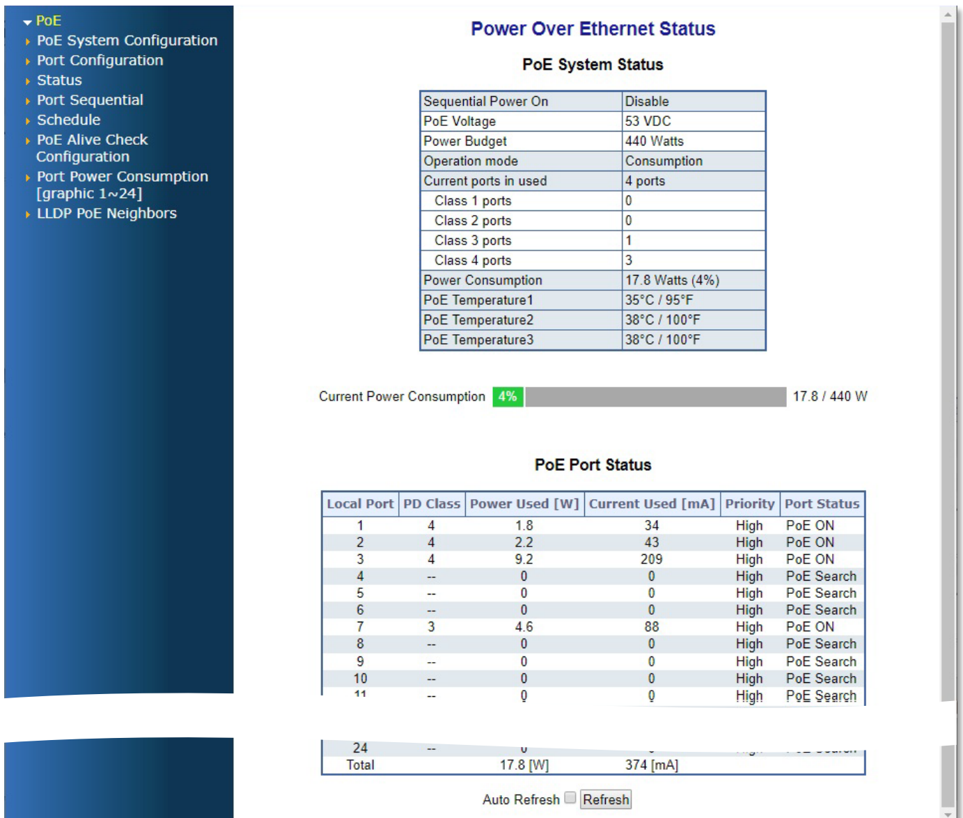
Figure 4-7-1-1: Power over Ethernet Status
