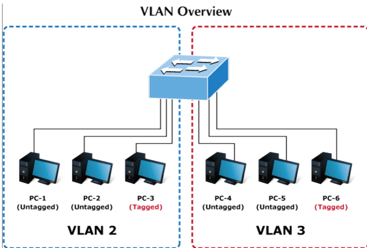
Figure 4-3-3-8: Two Separate VLANs Diagram
