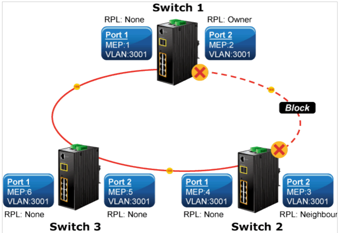
Figure 4-8-6: Ring Example Diagram
