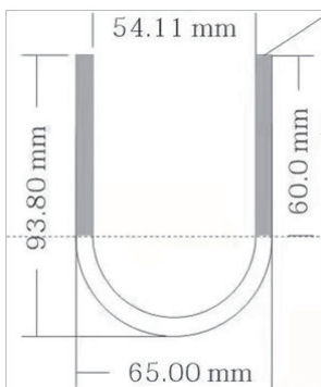
U-bolt Dimensions
