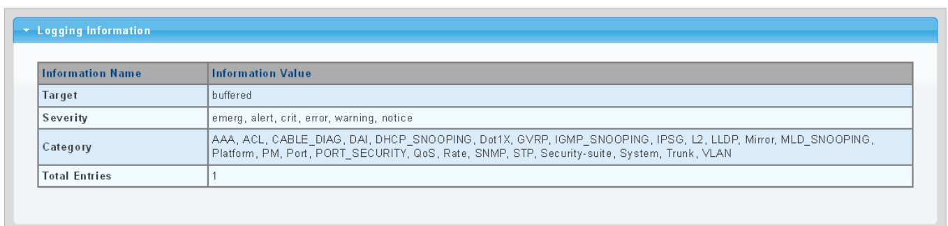
Figure 4-2-9-8: Logging Information Page Screenshot
