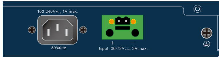
Figure 2-1-4-1: AC inlet power socket
