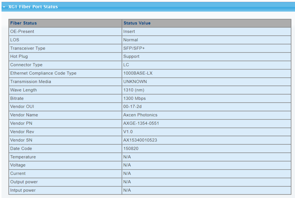
Figure 4-3-10-2: Fiber Port Status Page Screenshot
