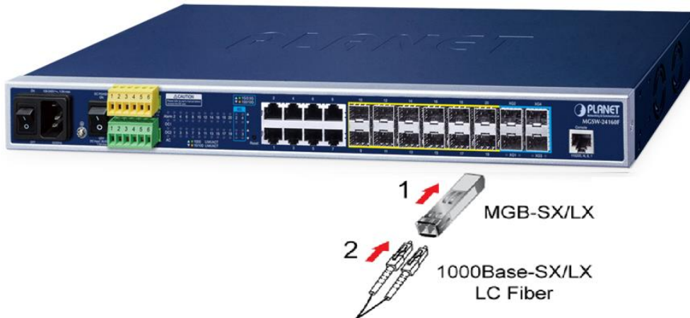
Figure 2-3-1-1: Plug in the SFP/SFP+ Transceiver
