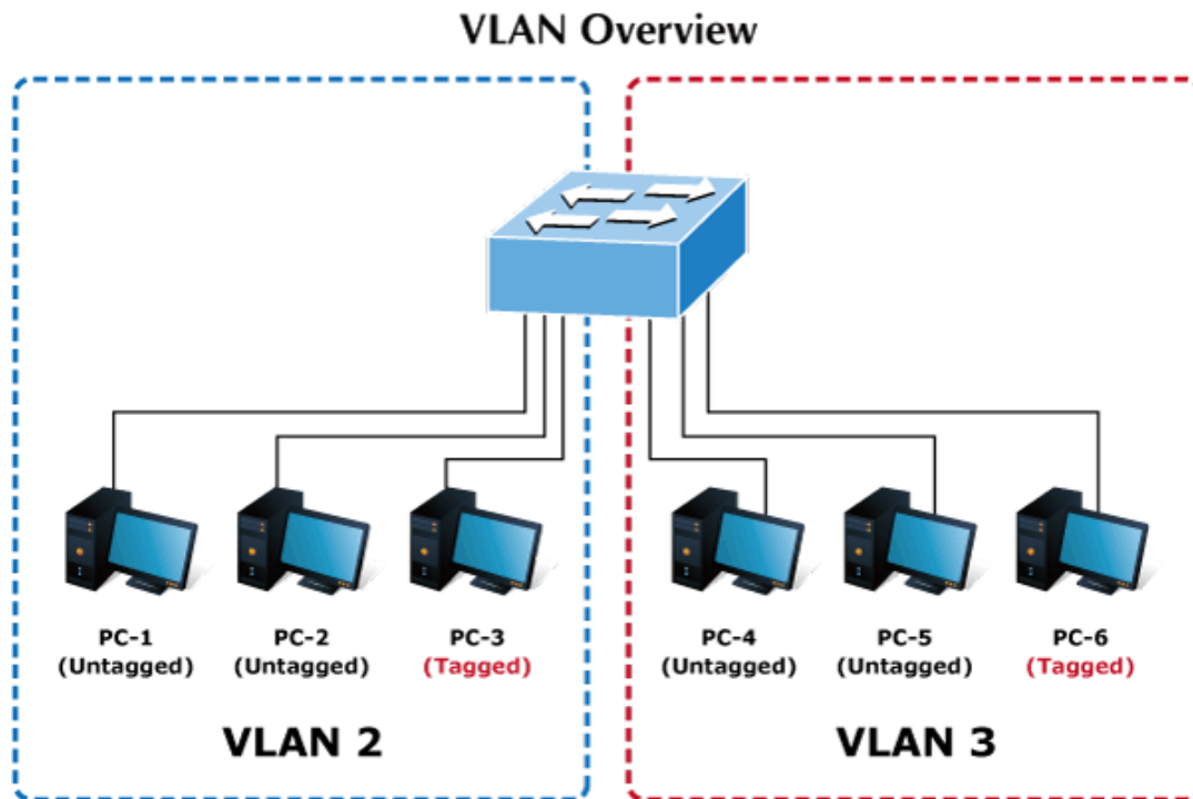
Figure 4-5-14-1: Two Separate VLAN Diagrams
