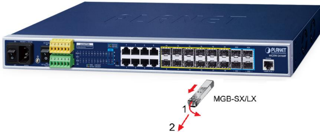
Figure 2-3-2-1: Pull out the SFP Transceiver Module
