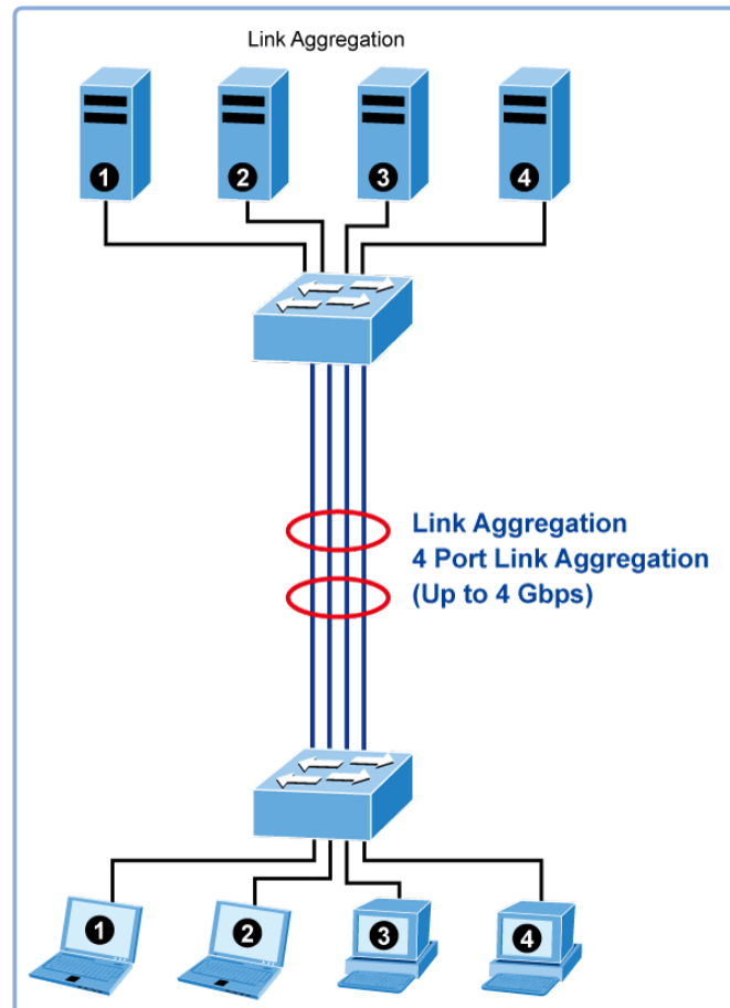
Figure 4-4-1: Link Aggregation
