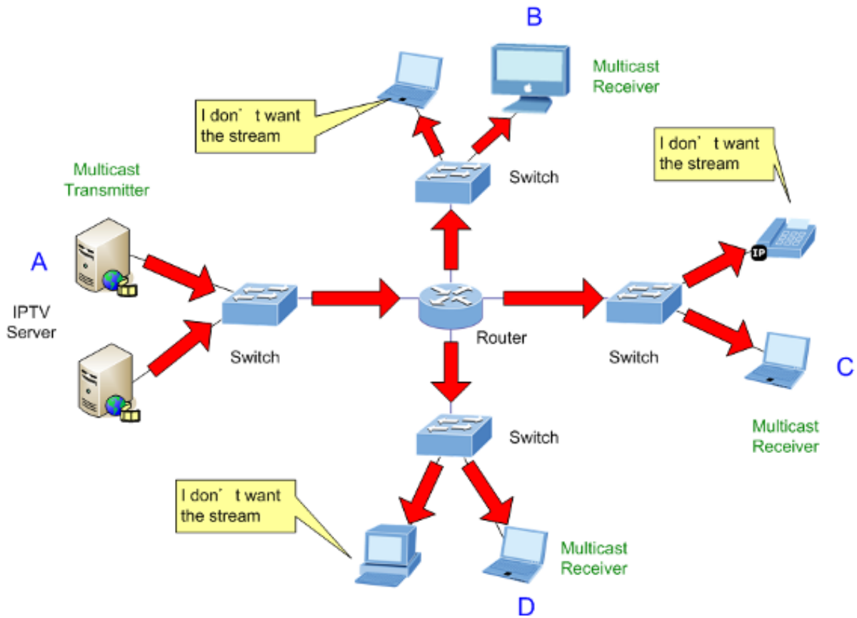
Figure 4-8-2: Multicast Flooding
